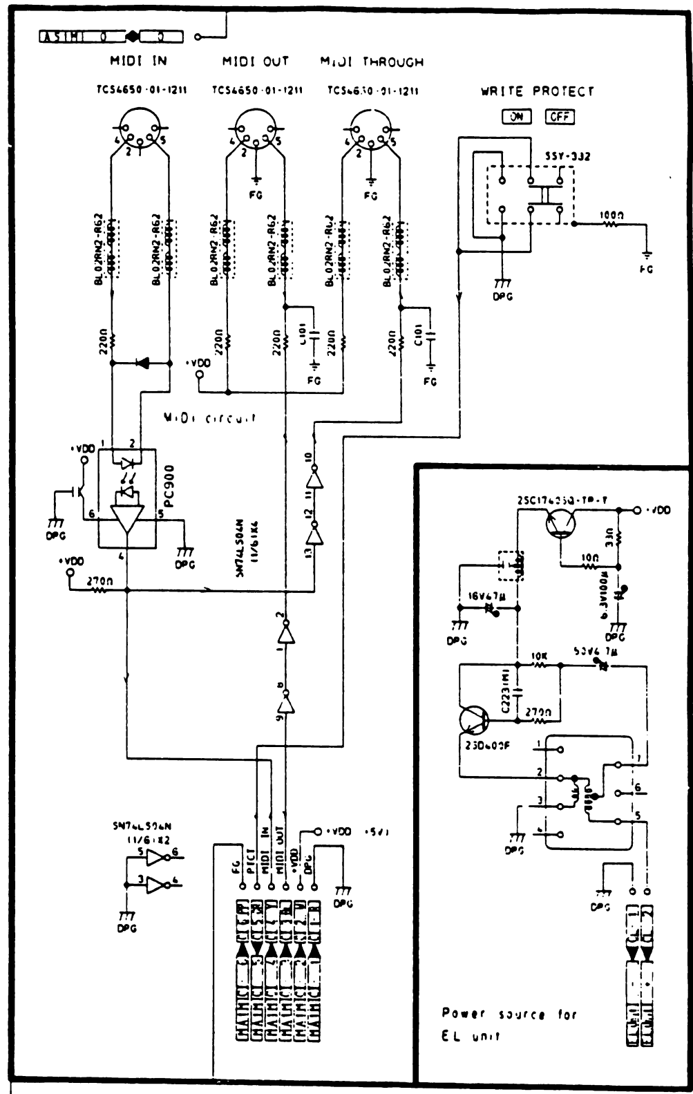
PCB-M5154-MA3M
